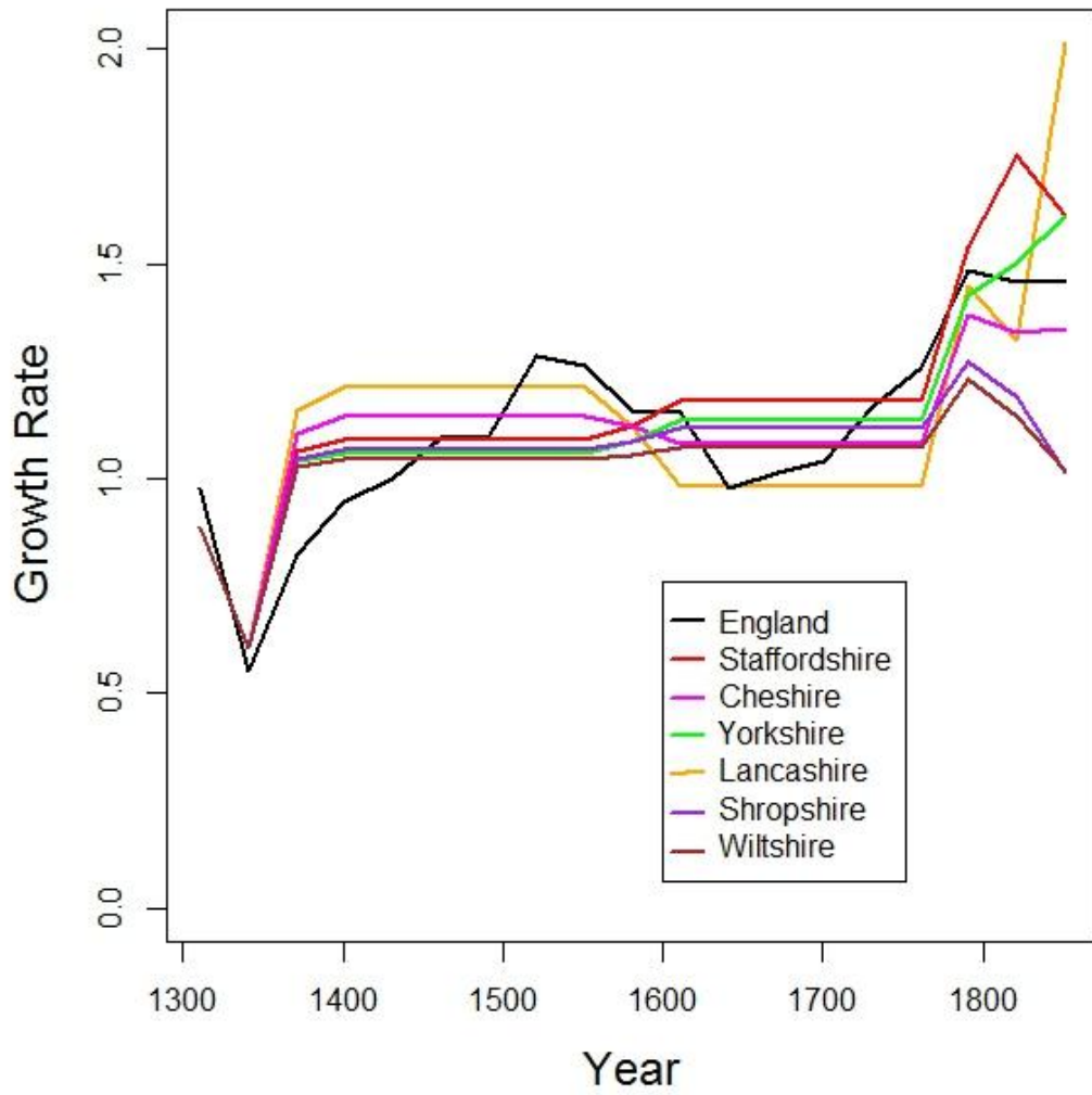
Figure 18: Population growth rates for the six counties in Figure 6.
