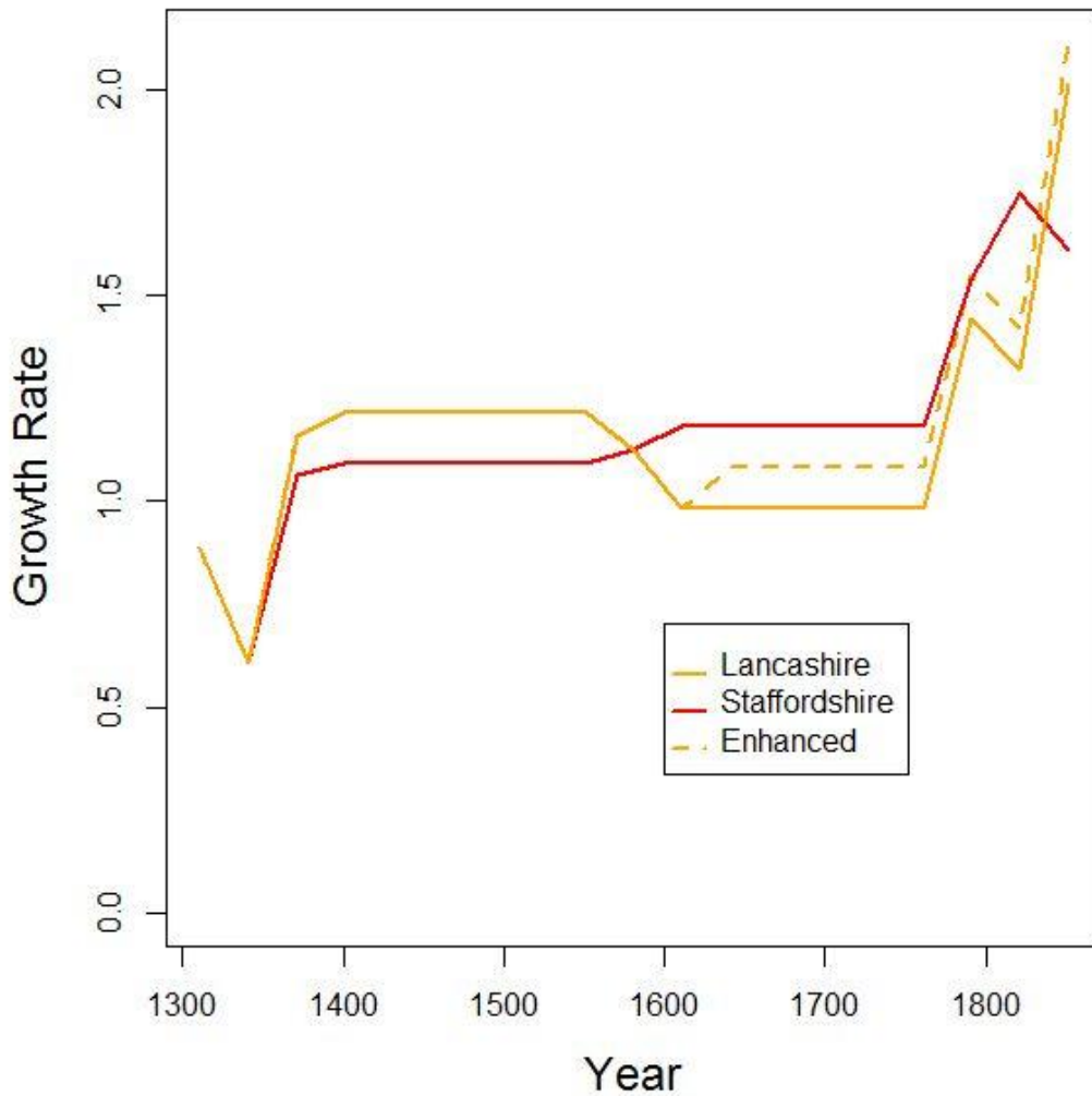
Figure 22: Population growth rates relevant to Plant and Sykes.
