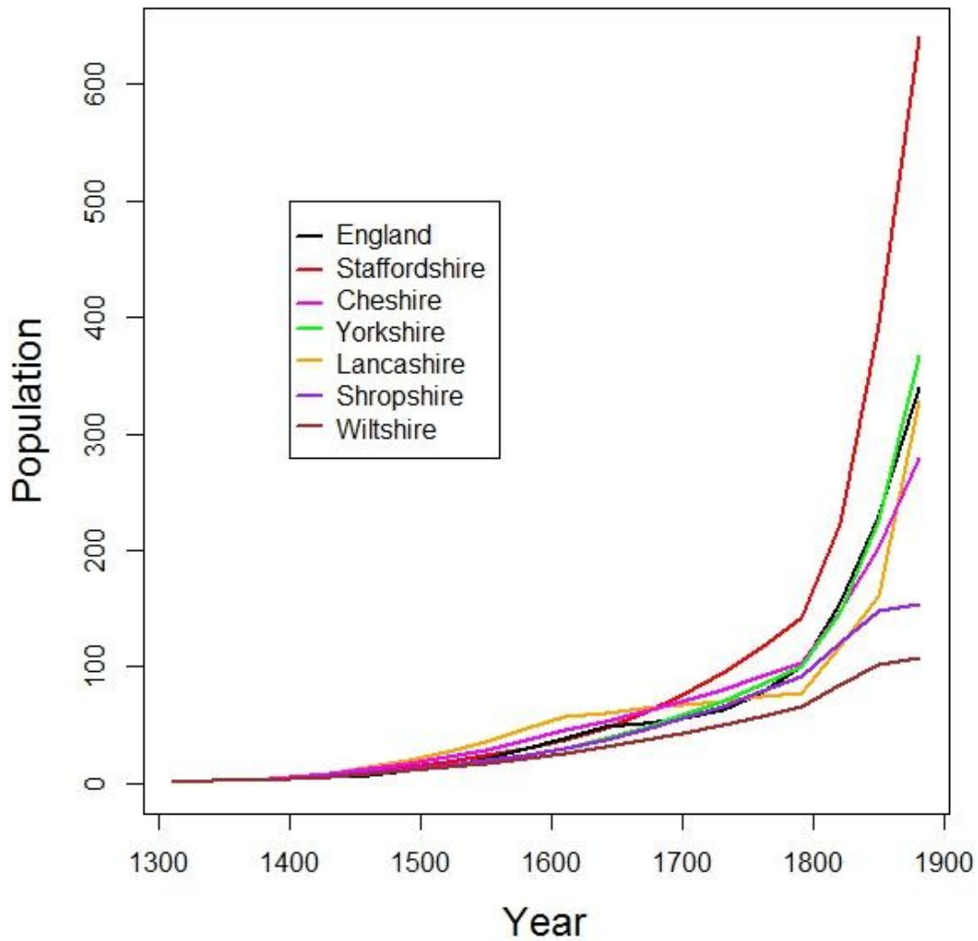
Figure 19. Population growth curves of the means of the largest 0.1% of the simulated lines in each of the six counties, together with the corresponding mean using the base England parameters.
